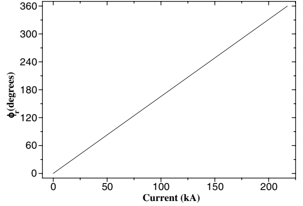
Figure 2. Sensor transfer function: relative phase versus applied current.
